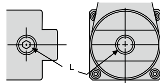
AIR INLETS, SINGLE DIRECTION MOTORS
